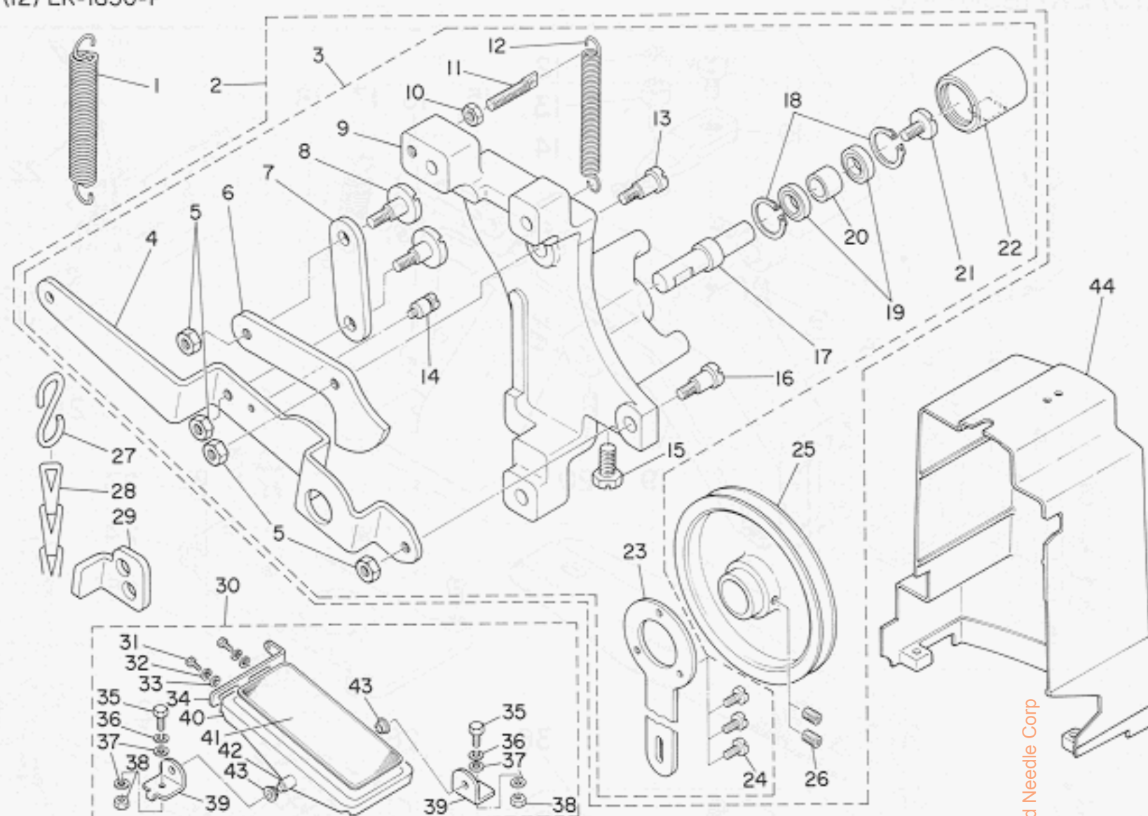
(12) LK-1850-P PEDAL TYPE CLAMP FOOT LIFTING DEVICE 足踏式押え上げ装置
